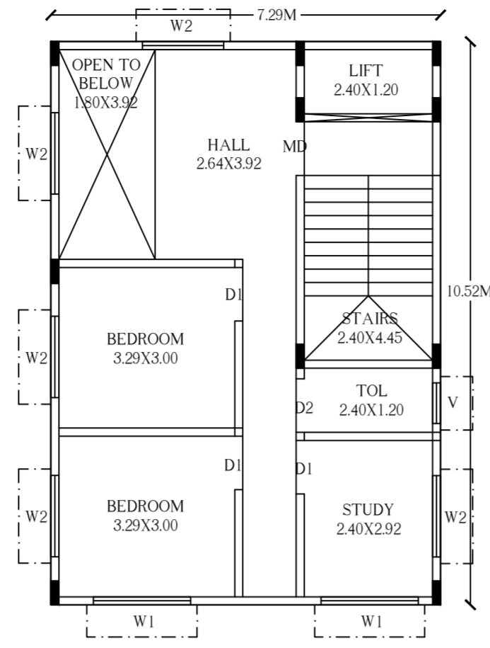
TYPICAL FIRST & SECOND FLOOR PLAN
